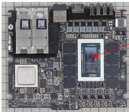
Main PCB
