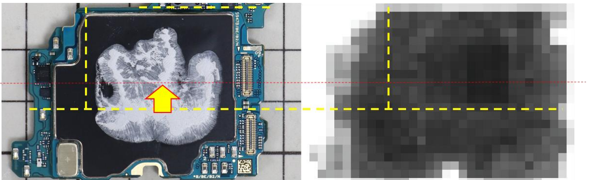
Cross-sectional position
